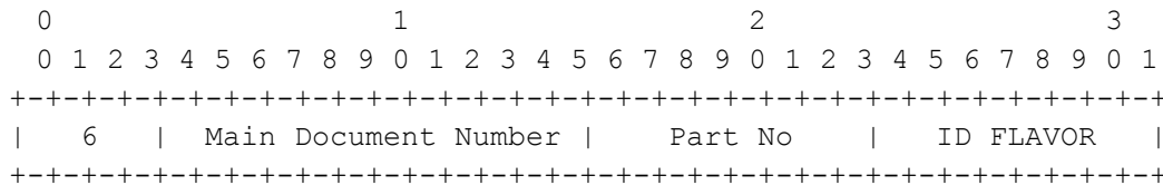
Figure 10: Payload Format Descriptor ATSC Standards
