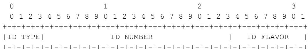
Figure 6: The Payload Identification Field
