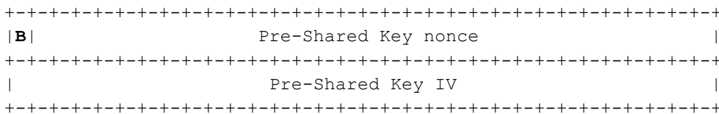
Figure 25: Pre-Shared Key nonce field with Odd/Even Bit B
