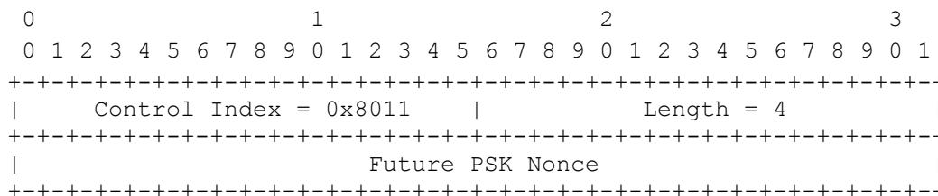
Figure 20: PSK Future Nonce Announcement Message
