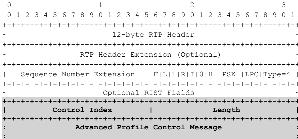
Figure 12: Control Message Format
