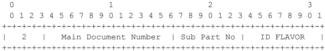
Figure 8: Payload Format Descriptor for SMPTE Standards
