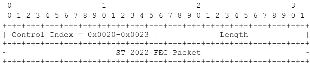
Figure 16: ST 2022 FEC Control Message
