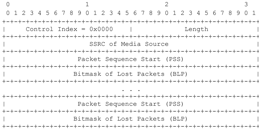
Figure 13: NACK Bitmask Control Message
