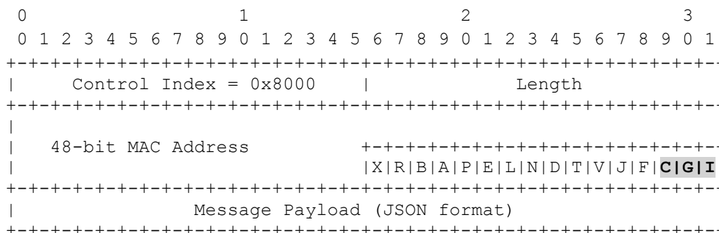
Figure 17: Main Profile Keep Alive Control Message
