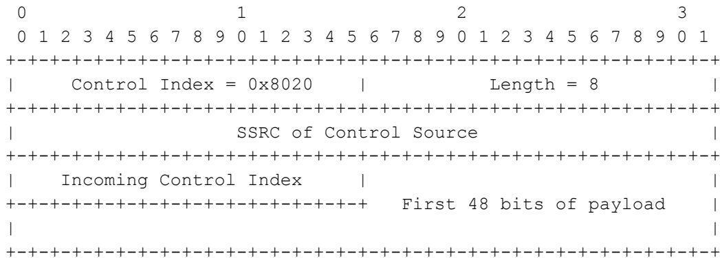
Figure 21: Control Message Unsupported Response
