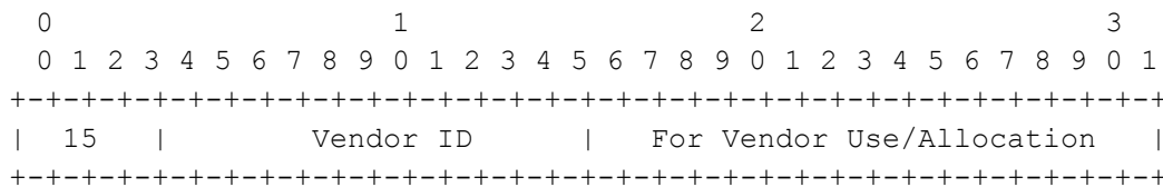
Figure 11: Payload Format Descriptor for the Vendor-Defined Category
