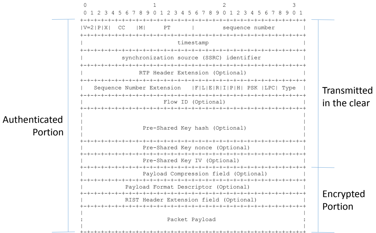
Figure 23: Clear, authenticated and encrypted fields using PSK
