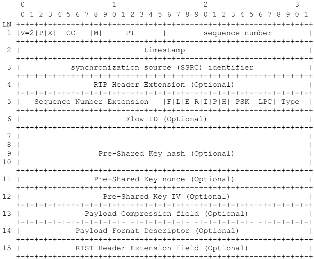
Figure 1: RTP Header for Tunnel Packets
