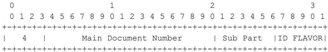
Figure 9: Payload Format Descriptor for ISO/IEC Standards
