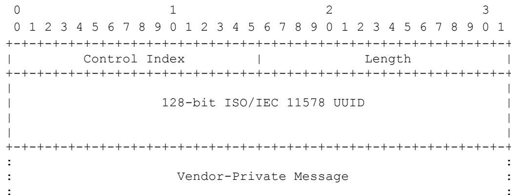
Figure 22: Vendor Private Control Message Format
