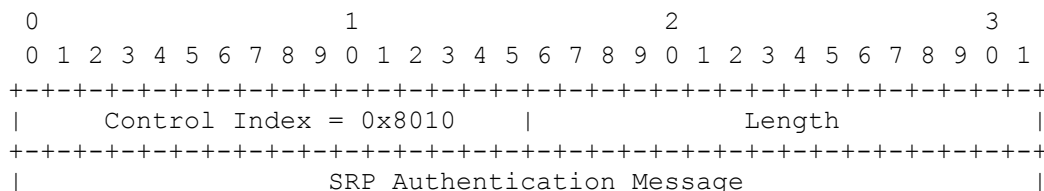
Figure 19: Advanced Profile Flow Attribute Control Message
